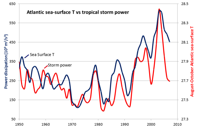
Figure 19.3.3 Relationship between Atlantic tropical storm cumulative annual intensity and Atlantic sea-surface temperatures.
