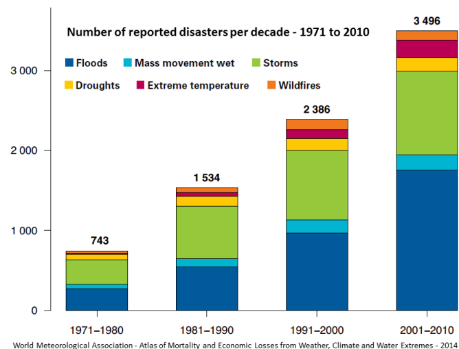
World Meteorological Association - Atlas of Mortality and Economic Losses from Weather, Climate and Water Extremes - 2014 Figure 19.3.8 Numbers of various types of disasters between 1971 and 2010. [Image Description]
